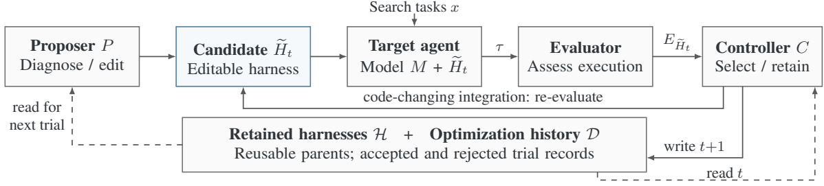
Figure 1: One harness-improvement trial. Solid arrows carry artifacts or updates; dashed arrows read retained state. Task-agent memory inside H differs from optimization history \mathcal{D} . Code-changing integration requires re-evaluation. Recursive scope is assessed separately in Section 3.
