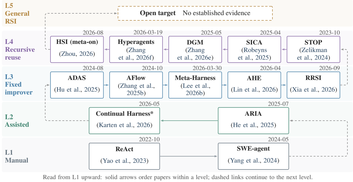
Figure 2: Selected configurations grouped by the five levels of Liu et al. (2026d). Within each level, arrows follow first arXiv release; cross-level links indicate reading order, not chronology or technical inheritance. Dates may differ from citation years; spacing is schematic. *Continual Harness denotes its human-guided GPP configuration. Higher recursive scope need not appear later: early L4 examples coexist with recent L3 methods. L5 remains an open target.
