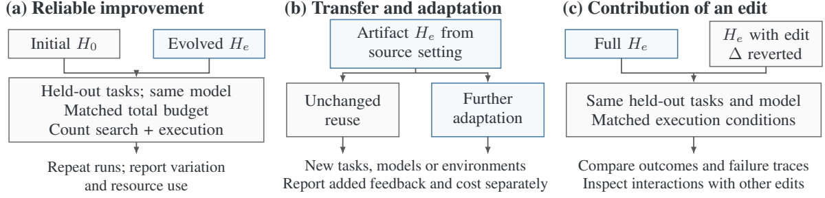
Figure 12: Conceptual evaluation comparisons; H_e is a selected evolved harness. Reliability, transfer, and edit attribution require different controls; track regressions and safety violations. Adaptation feedback must remain separate from final test evidence. A changed improver additionally requires a comparison of subsequent improvement, as discussed in Section 3.2.
