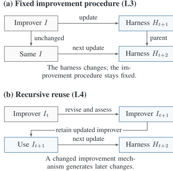
Figure 5: Fixed versus recursively reused improvement mechanisms. In (a), the same improver I produces successive harness revisions. In (b), an updated I_{t+1} is retained and invoked for later modification. This distinguishes L4 from L3 under Liu et al. (2026d); fixed outer constraints may remain. The schematics establish neither measured gains nor general recursion.
